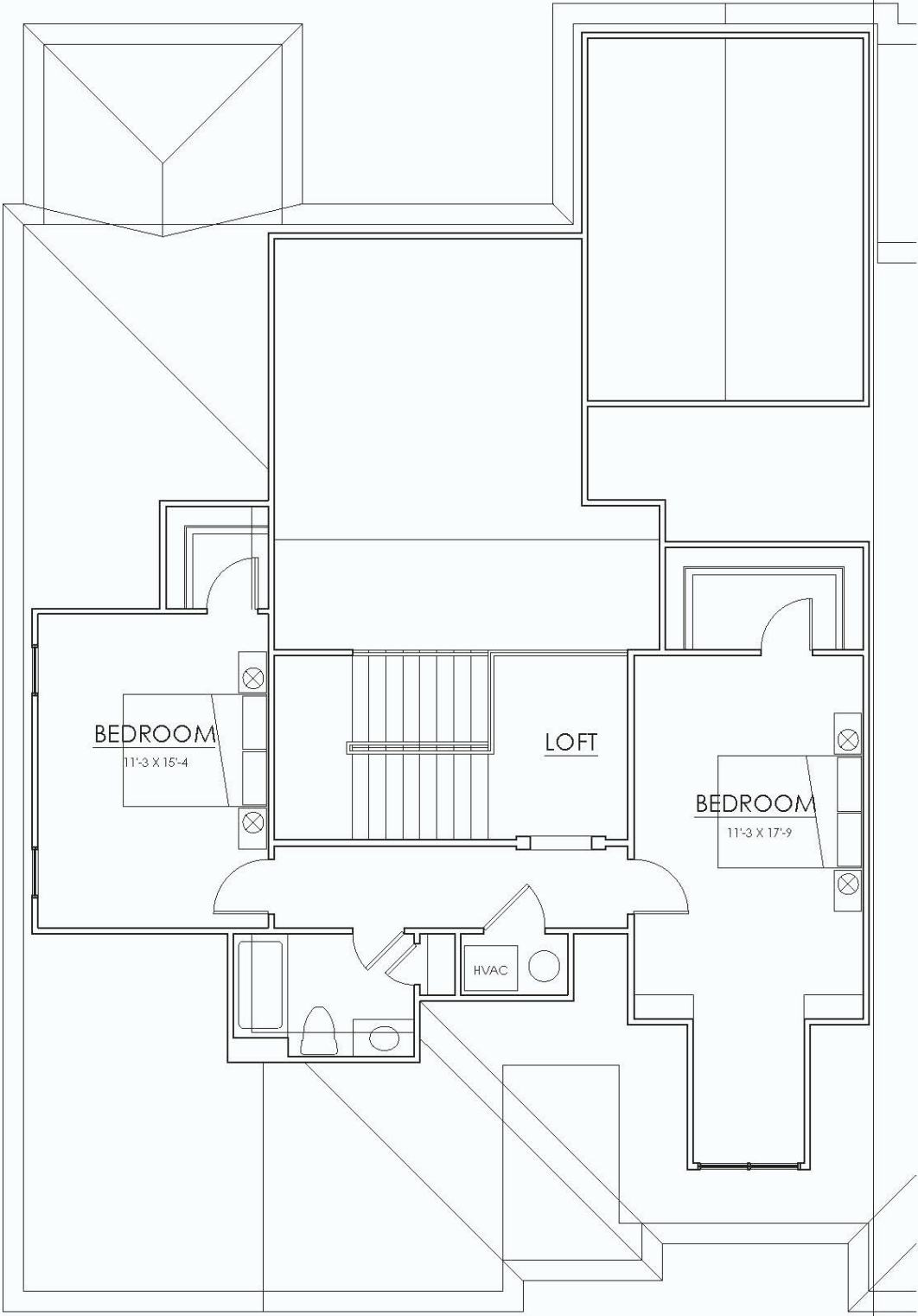
727 S.F. SECOND FLOOR PLAN
